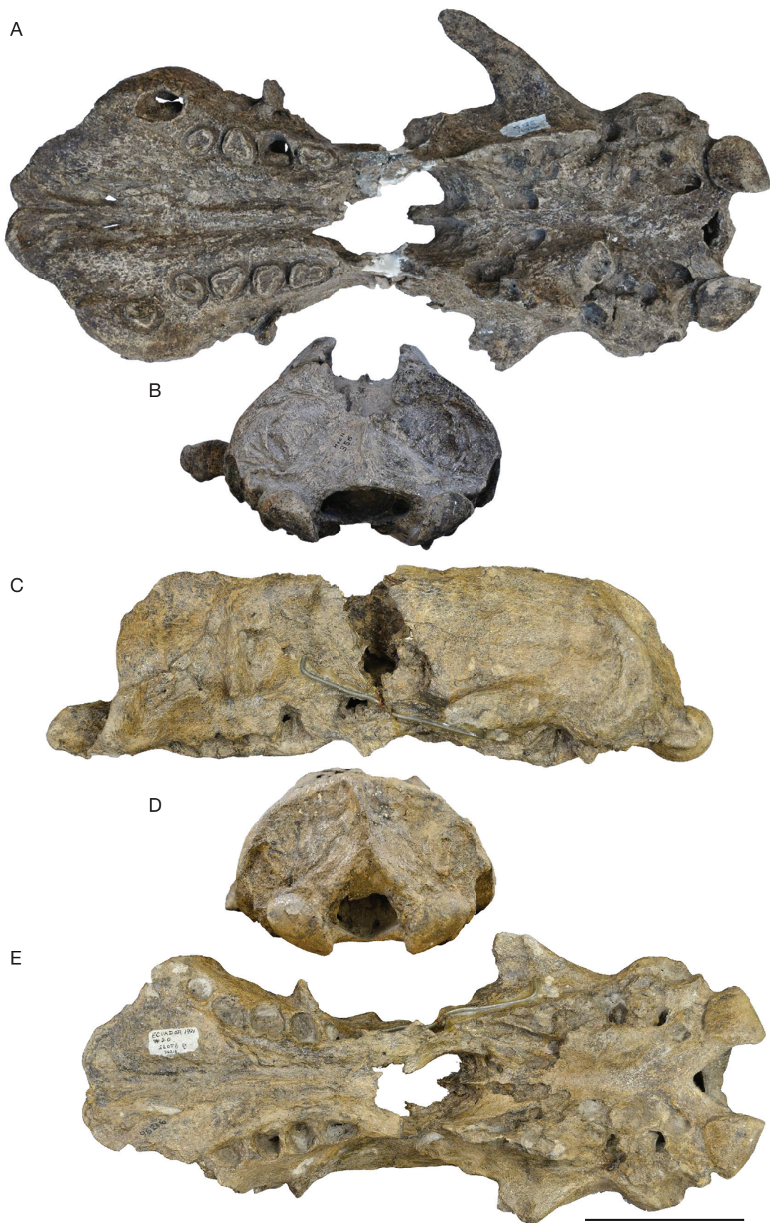
APPENDIX 3. — Skulls of Glossotherium wegneri (Spillmann, 1931) representing a robust ( A, B ) and a gracile ( C-E ) morph, which are suggestive of the presence of sexual dimorphism: A, B , skull (MECN 356) in ventral ( A ), and posterior ( B ) views; C-E , skull (AMNH 96216) in lateral ( C ), posterior ( D ) and ventral ( E ) views. Scale bar: 10 cm.
