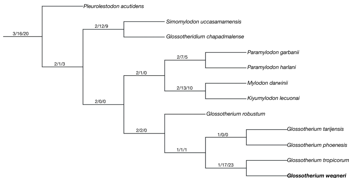
FIG. 5. — Single most parsimonious tree (tree length = 1167 steps; consistency index = 0.545; retention index = 0.887) showing the phylogenetic relationships among Mylodontini and the phylogenetic position of the mylodontid sloth Glossotherium wegneri from the Pleistocene of Ecuador within the clade. Numbers at each node represent Bremer, bootstrap, and jackknife support values, respectively. The complete matrix and tree, that resulted from the present phylogenetic analysis, are available in Appendices 5; 6.
