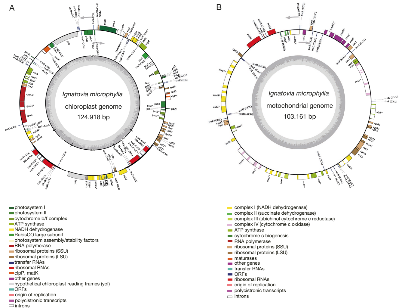
Fig. 2. — Circular genome maps of the plastome (A) and mitogenome (B) of Ignatovia microphylla (Ignatov & Ignatova) U.B.Deshmukh. Genes shown on the outside of the circle are transcribed clockwise, whereas those on the inside are transcribed counter-clockwise. The asterisk * indicates intron-containing genes.
