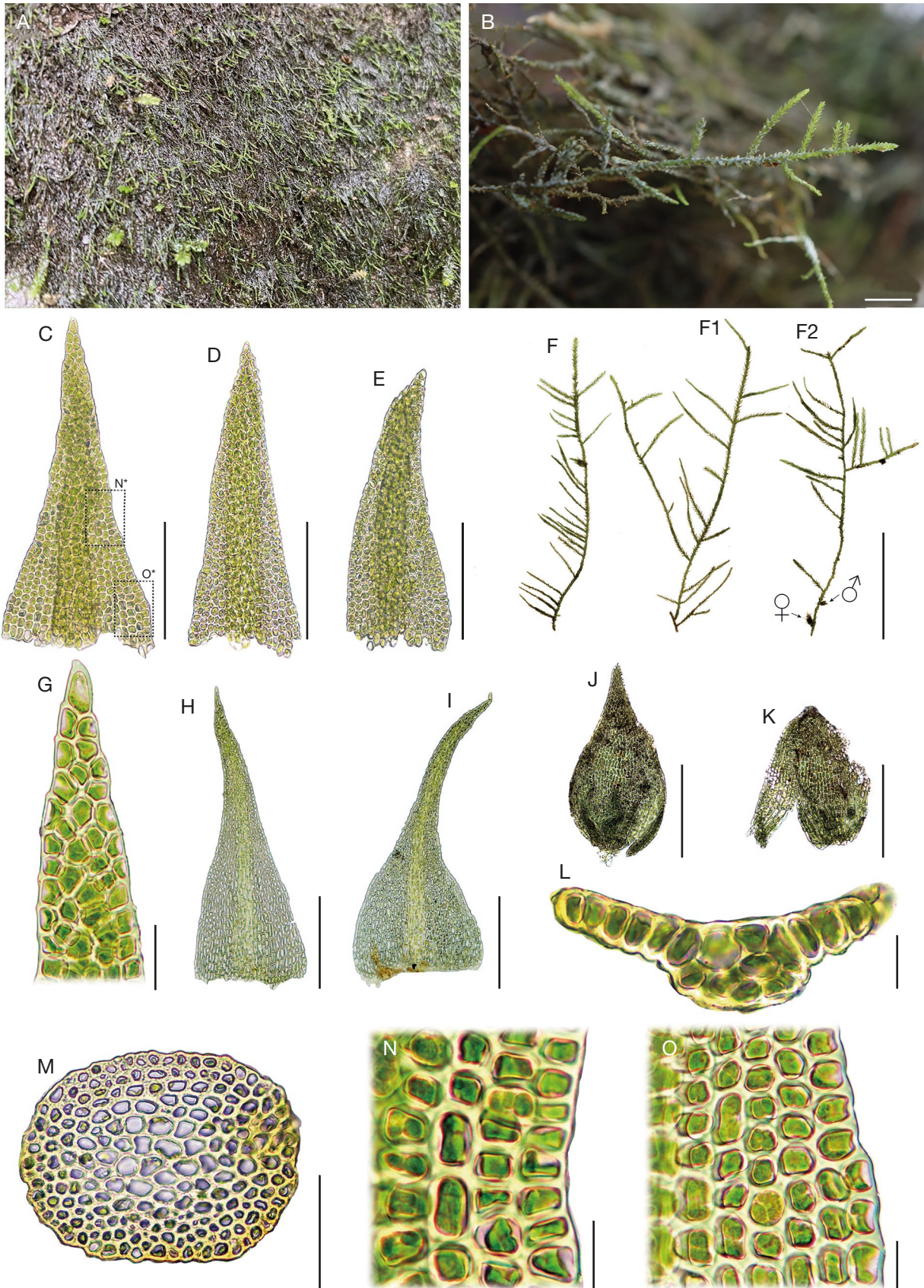
FIG. 3. — Ignatovia microphylla (Ignatov & Ignatova) U.B.Deshmukh: A , field population on rock; B , closer view of plant; C , stem leaf; D , E , branch leaves; F , plants; G , apex of leaf; H , I , perichaetial leaves; J , K , perigonal leaves; L , cross section of leaf; M , cross section of stem; N , middle laminal cells; O , basal laminal cells. All from R.L. Zhu et al. 20240903-51 (HSNU, HTC). Scale bars: A, B, 2 mm; C-E, 100 \mu m; F, 5 mm; G, 20 \mu m; H-K, 200 \mu m; L, N, O, 10 \mu m; M, 50 \mu m.
