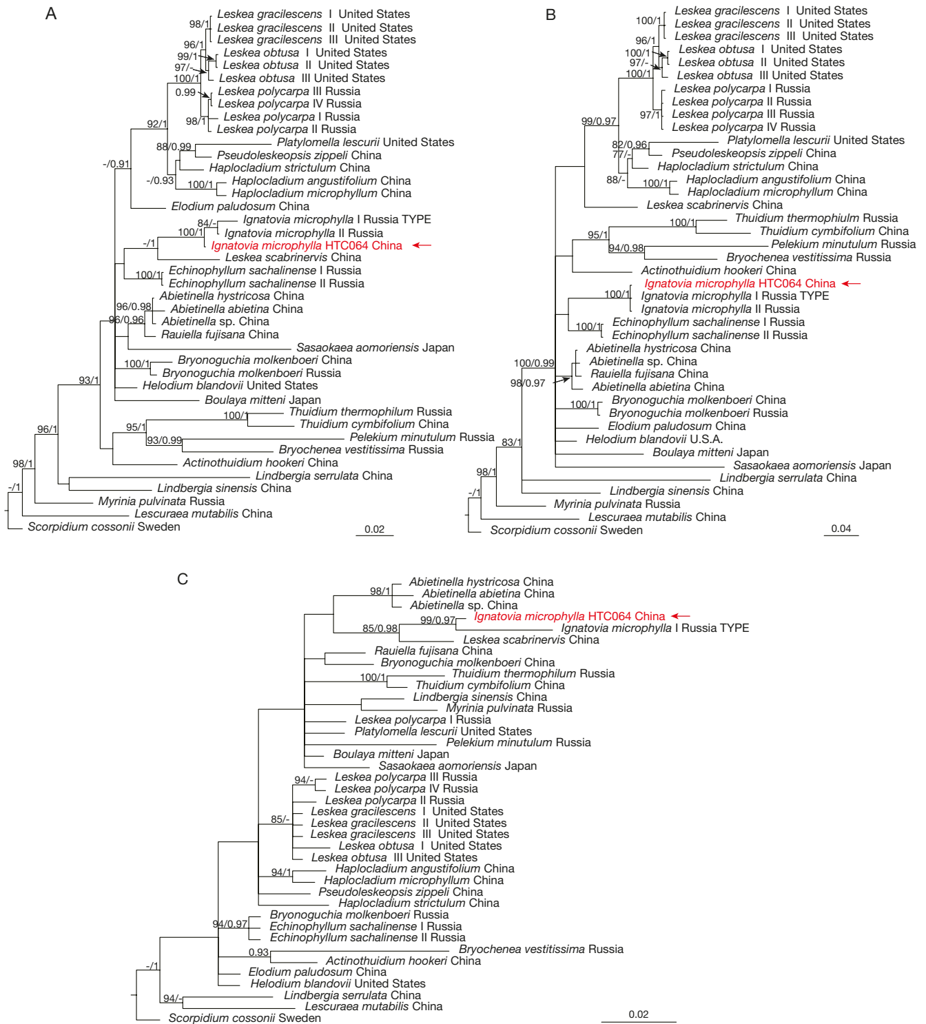
FIG. 1. — Phylogeny tree of Thuidiaceae and Leskeaceae species. The topology derived from the Bayesian tree is shown. A , phylogeny tree based on ITS + trnL-F dataset; B , phylogeny tree based on ITS dataset; C , phylogeny tree based on trnL-F dataset. ML bootstrap values BS ≥ 75 are shown at left and Bayesian posterior probabilities values PP ≥ 0.95 at right. The newly sequenced Chinese accessions are marked in arrows.
