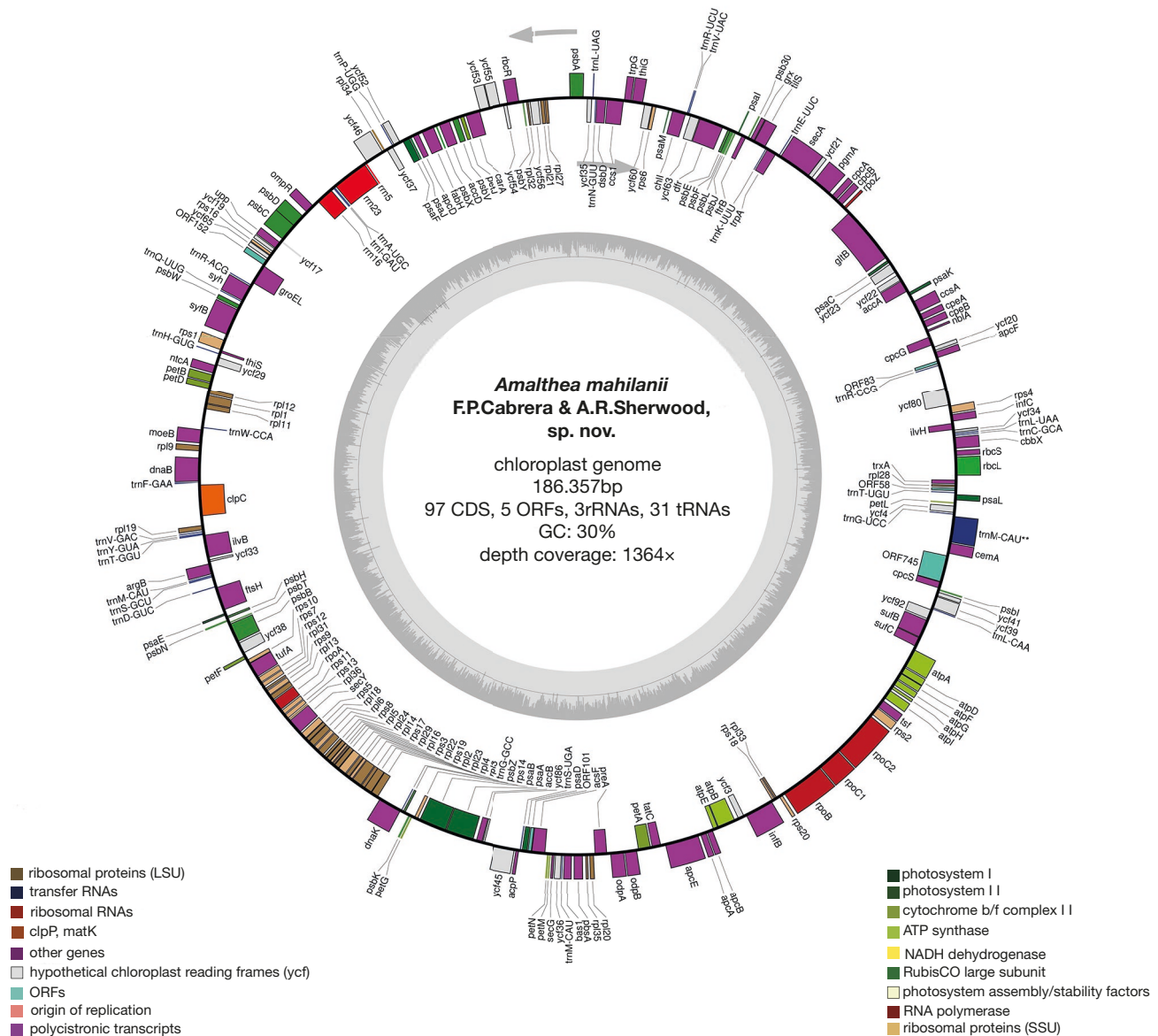
FIG. 2. — Chloroplast genome (CP) of Amalthea mahilani F.P.Cabrera & A.R.Sherwood, sp. nov. (ARS 09490, GenBank PP777198, 1364x coverage). Overview of the chloroplast genome features. Genes outside the circle are transcribed clockwise, while genes inside are transcribed counter-clockwise. Functional groups are color-coded. Inner circles represent Guanine-Cytosine (GC) and Adenine-Thymine (AT) content.
