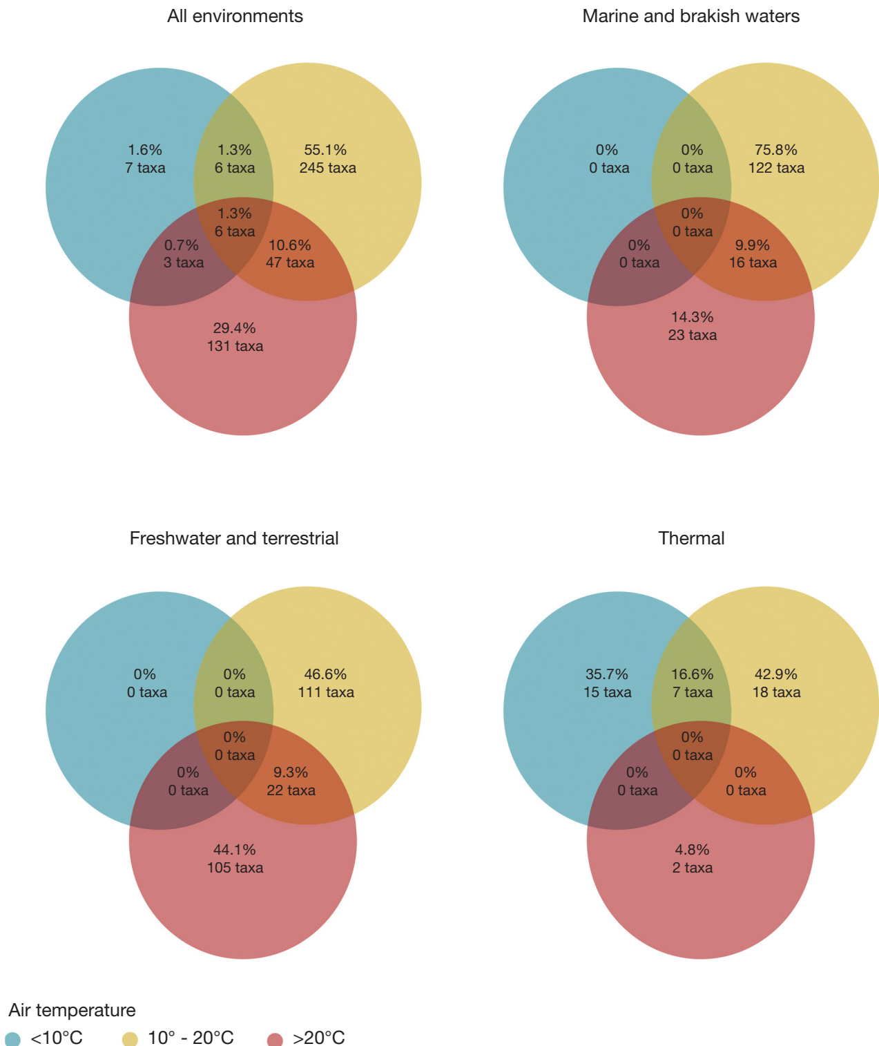
FIG. 4. — Percentage of common and unique cyanobacteria species by islands grouped according to their annual mean air temperature. “<10°C”: Iceland; “10-20°C”: Azores, Madeira, Canary Islands, and Brazilian coastal islands; “>20°C”: Bahamas, Cuba, Puerto Rico, United States Virgin Islands, Cape Verde, and Curaçau.
