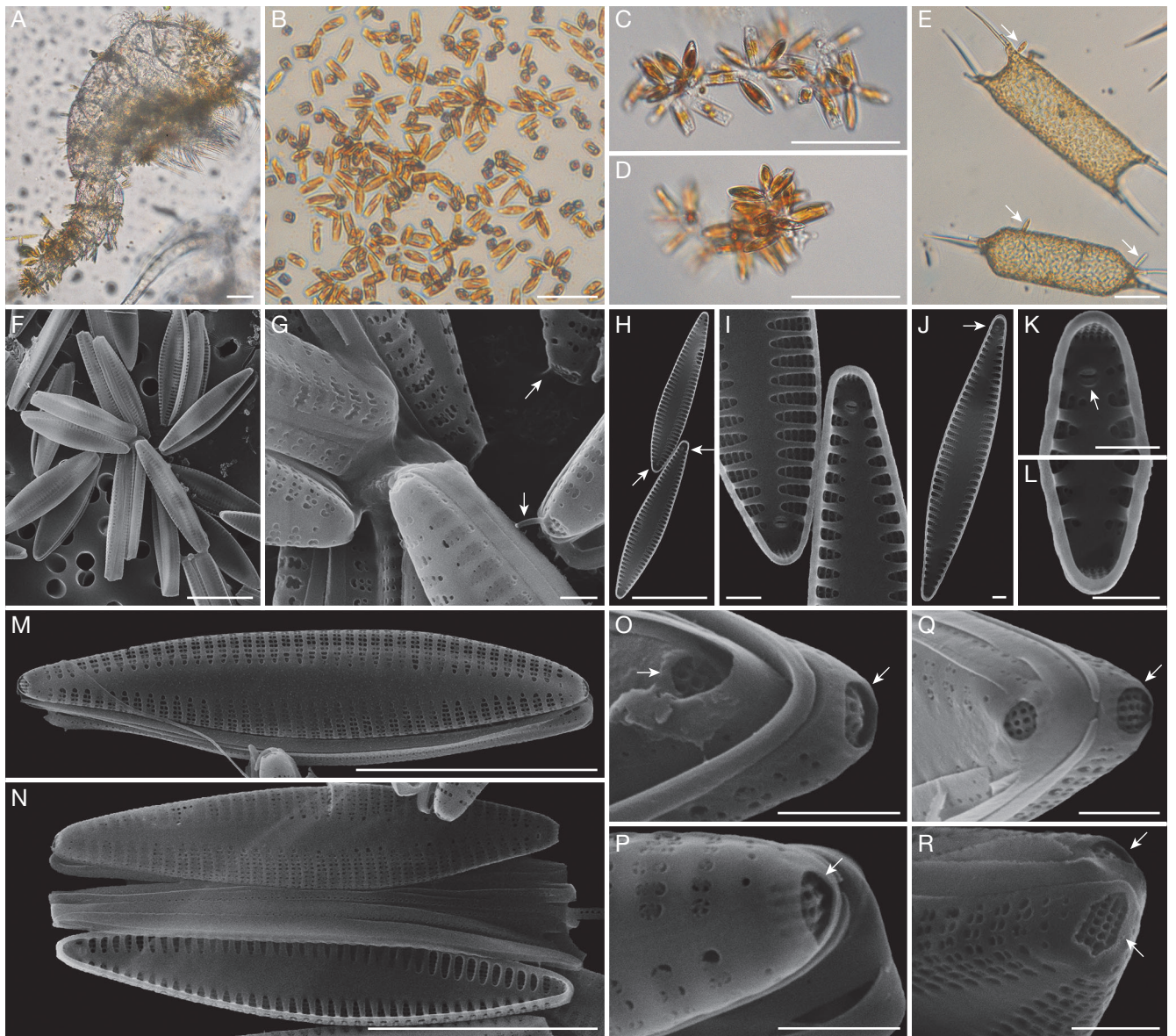
FIG. 3. — Light (A–E) and scanning electron (F–R) micrographs of Tabularia parva (Kützinger) D.M. Williams & Round: A, wild cells on the empty carapace of a copepod from the port of Brest, Brittany; B–R, cultured cells; B, note a part of the cells arranged perpendicularly to bottom; C, D, cells forming bunches attached to an exopolymeric transparent particle; E, the arrows indicate cells attached to the diatom Trieres chinensis (Greville) Ashworth & E.C. Theriot; F, G, cells attached by mucilage pads; G, the arrows indicate the thin mucilage; H–R, acid-cleaned valves; H–L, internal view of the valve. The arrows indicate the single rimoportula per valve; M, N, valve view; O–R, the arrowheads indicate the ocellulimbus. Scale bars: A–E, 50 µm; F, H, M, N, 10 µm; G, I–L, O–R, 1 µm.
