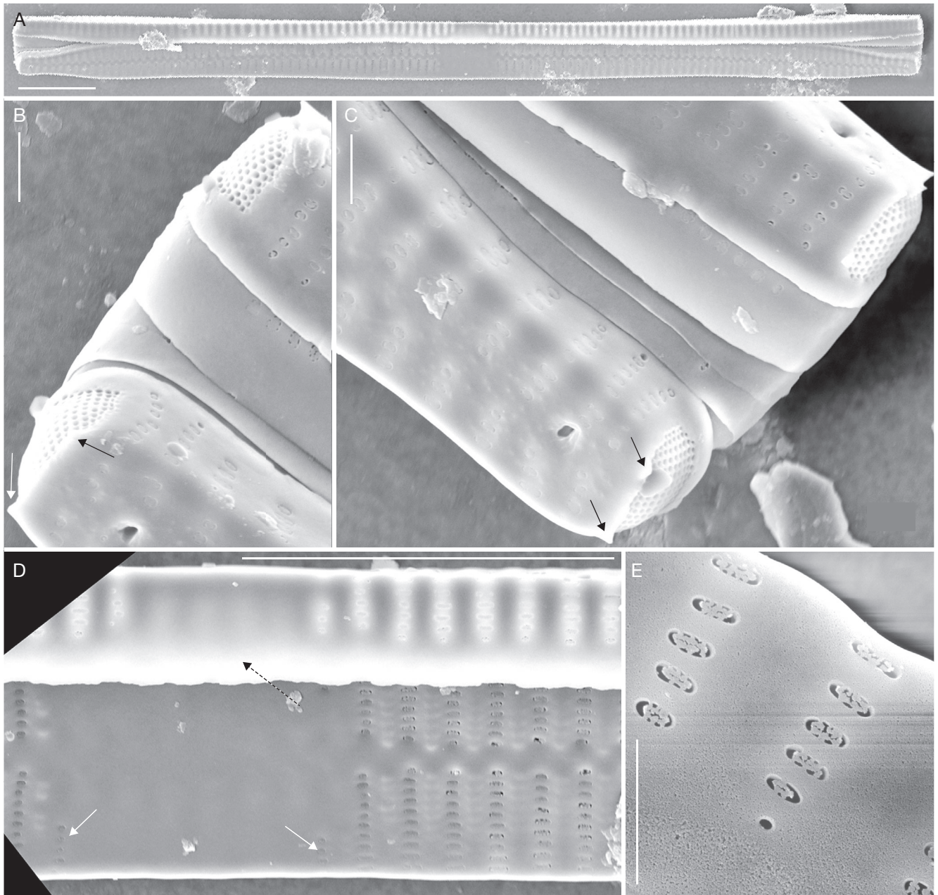
FIG. 15. — Ulnaria dongtingensis Bing Liu, sp. nov., SEM, girdle view: A , a separated frustule; B , C , two apices of A showing the closed girdle bands, ocellulimbi, and two horn-like projections (arrows) overhang the ocellulimbus; D , detail of A , note two shortened striae bordering the central area (two arrows) and hyaline mantle middle part (dashed arrow); E , a detail of the closing plates on the mantle. Scale bars: A , D , 10 \mu\text{m} ; B , C , E , 1 \mu\text{m} .
