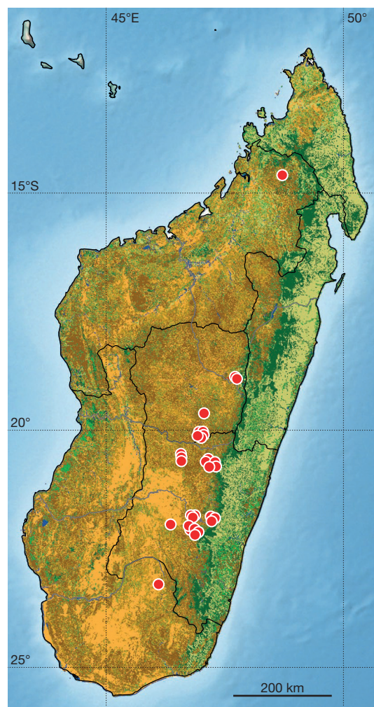
FIG. 44. — Distribution map of Benthamia flavida Schltr.
