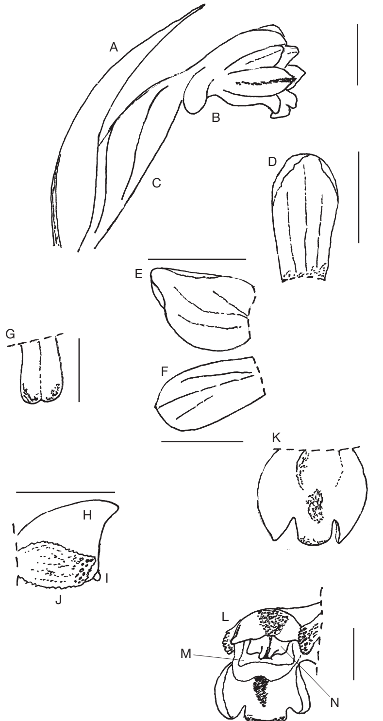
FIG. 2. — Sketch by Pascal Descourvières showing the different parts of a Benthamia A. Rich. flower: A , floral bract; B , profile of flower with spur; C , ovary; D , dorsal sepal; E , petal; F , lateral sepal; G , front view of spur; H , profile of column; I , rostellum; J , auricle; K , lip; L , front view of flower; M , stigmatic cavity; N , rostellum. Scale bars: A-F, H-L, 2 mm; G, 1 mm.
