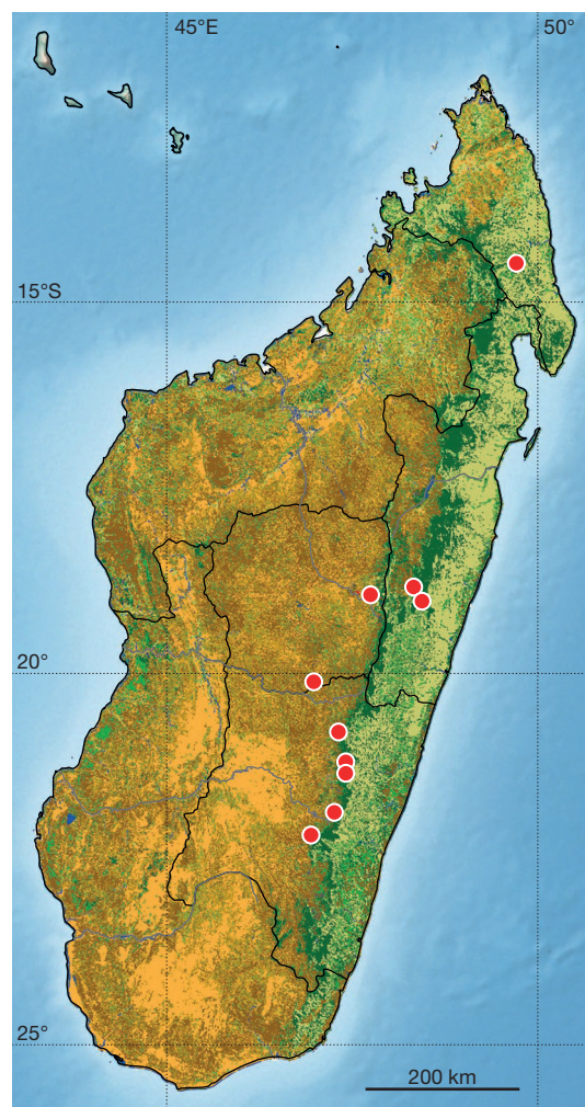
FIG. 50. — Distribution map of Benthamia herminoides Schltr.
