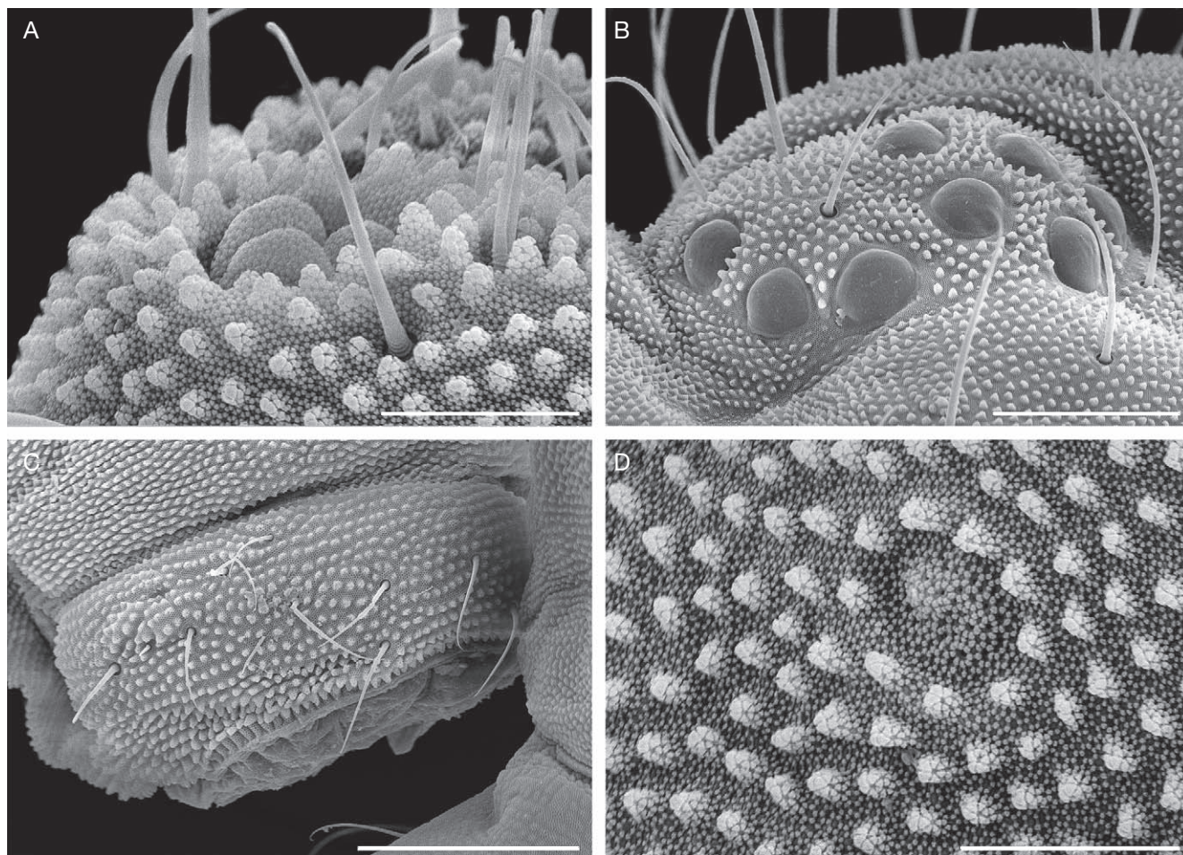
FIG. 4. — Friesea najtae n. sp. SEM microphotographs: A , tip of the antenna showing the trilobated apical vesicle; B , right side ocular patch showing eight ocelli and no PAO (front of the animal on the right side of the picture); C , ventral tube, lateral view; D , pseudopore on Abd. II. Scale bars: A, D, 10 \mu m; B, C, 50 \mu m.
